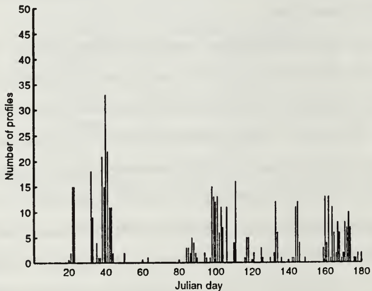
Figure 4.3 Number of Temperature Observations During Winter and Spring 1977, Illustrative of Typical Data Density in Any Given Half Year.
