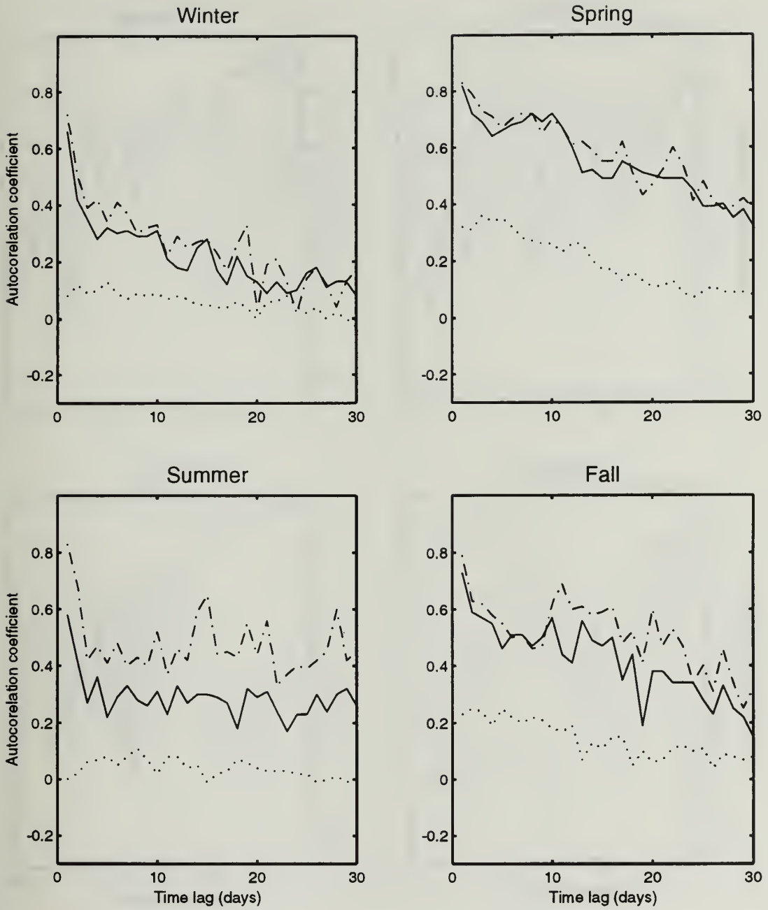
Figure D.3 Temporal Variations of Autocorrelation Function \eta(m, n) for Type II Data at 80% Water Depth. The Three Curves on Each Graph are the Dependency of \eta(m, n) on Time Lag n\Delta t for m = 0 (no lag, dash-dot), m = 1 (10 km lag, solid), and m = 15 (150 km lag, dots). Data were Obtained from the MOODS Temperature Data Base for the Years 1929 to 1991.
