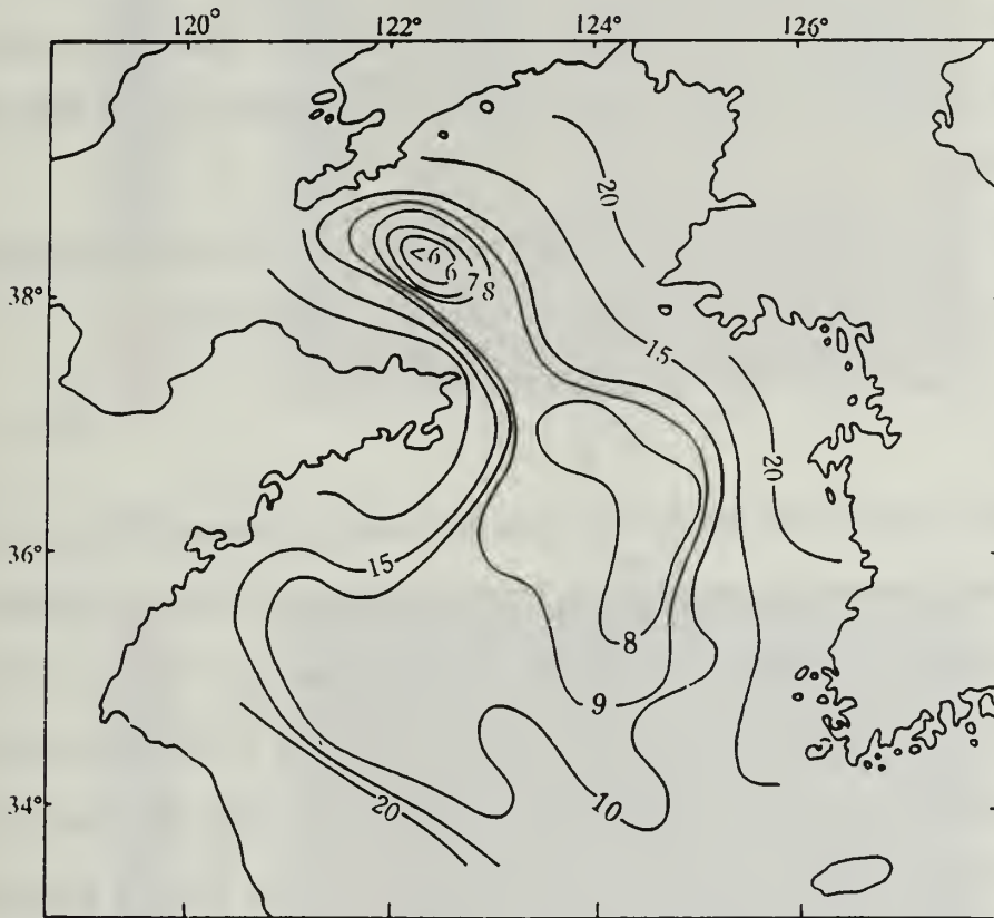
Figure 4.7 Temperature Distribution in Summer (April-November) of the 'Cold Water Mass of the Yellow Sea' (CWYS) Near the Sea Floor (from Su and Weng, 1994). Isotherms in Degrees Celsius.
