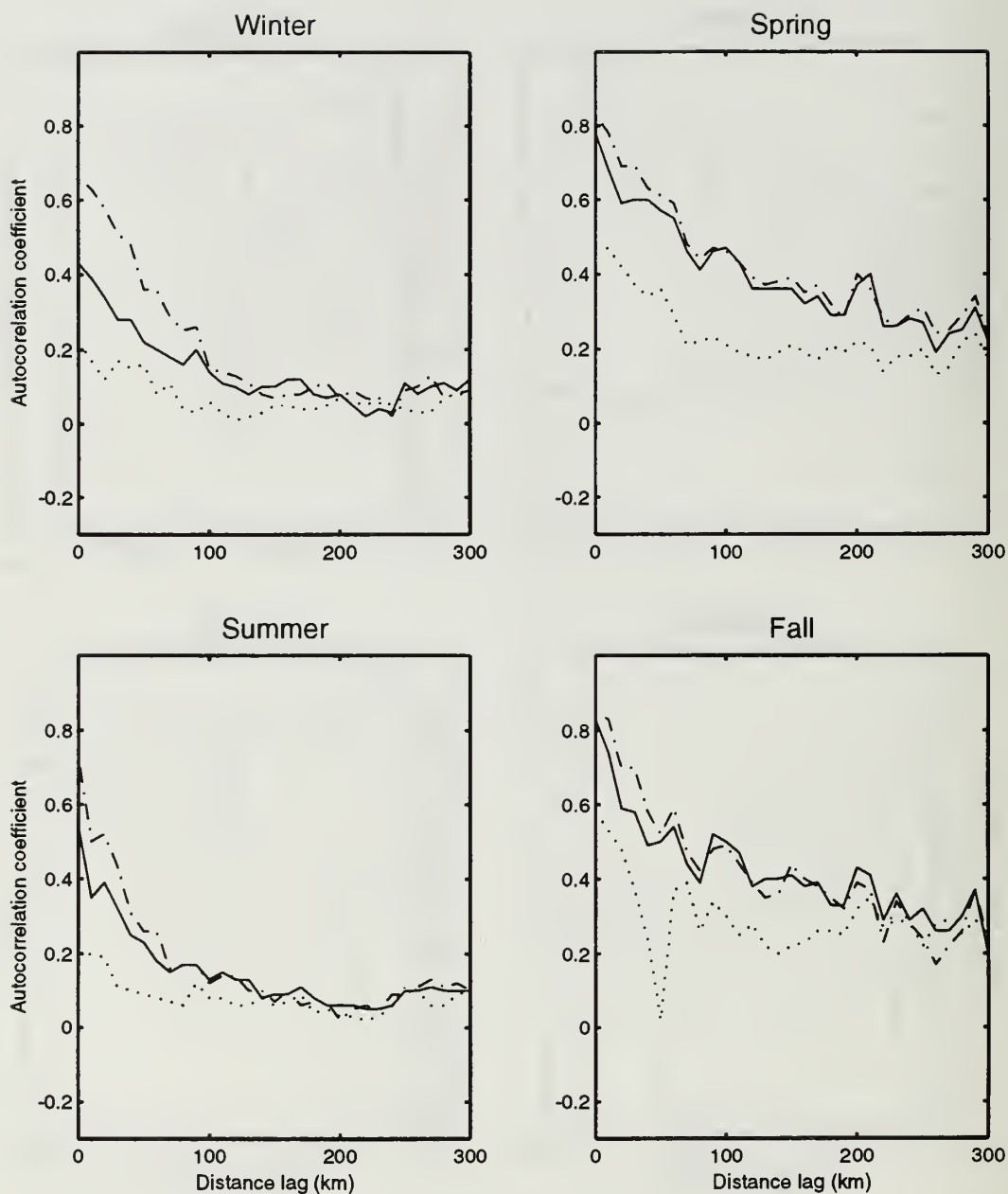
Figure D.8 Spatial Variations of Autocorrelation Function \eta(m, n) for Type II at 50% Water Depth. The Three Curves on Each Graph are the Dependency of \eta(m, n) on Spatial Lag ( m\Delta\gamma ) for n = 0 (no temporal lag, dash-dot), n = 1 (1 day lag, solid), and n = 15 (15 day lag, dots). Data were Obtained from the MOODS Temperature Data Base for the Years 1929 to 1991.
