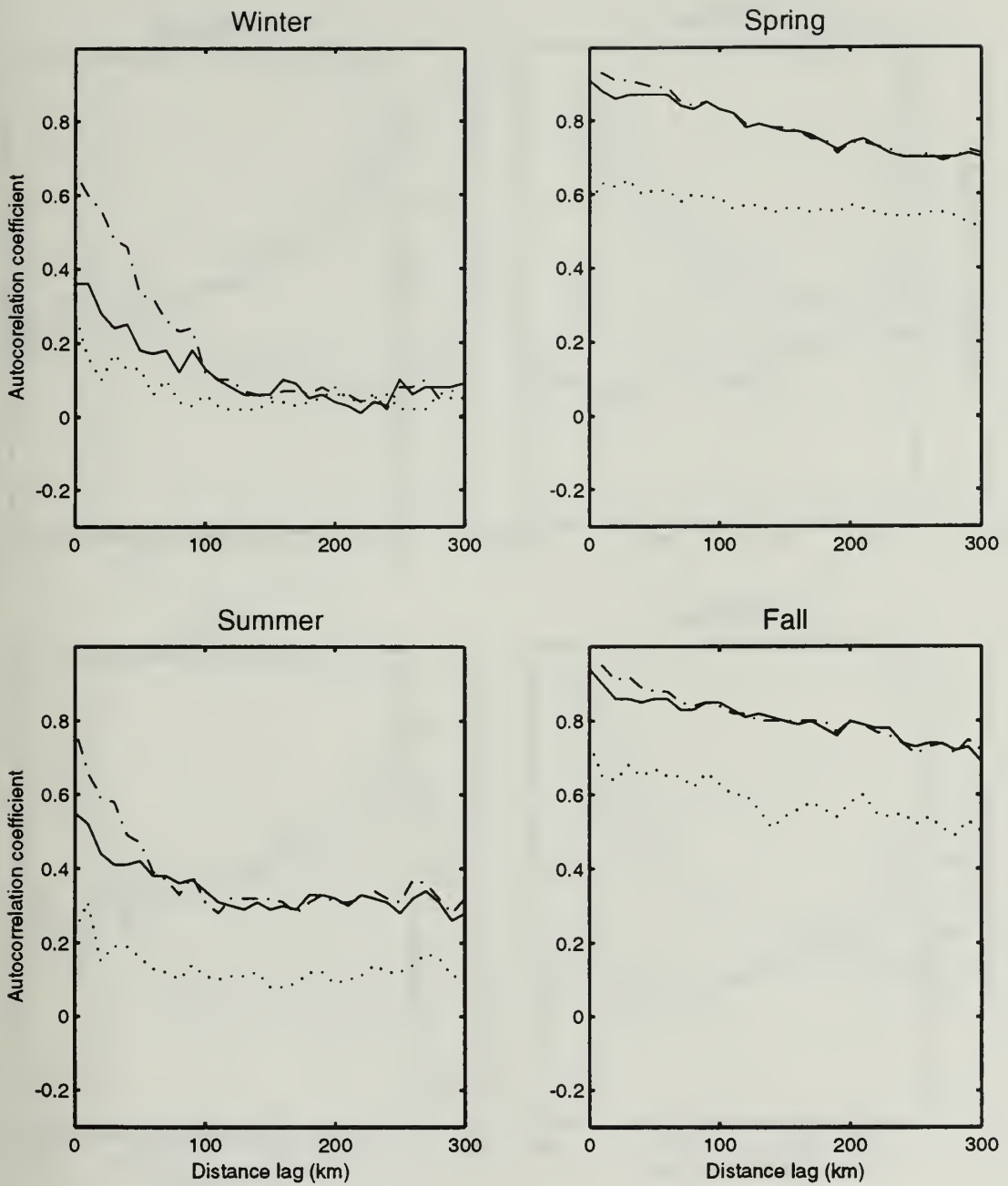
Figure D.7 Spatial Variations of Autocorrelation Function \eta(m, n) for Type II at the Surface. The Three Curves on Each Graph are the Dependency of \eta(m, n) on Spatial Lag ( m\Delta\gamma ) for n = 0 (no temporal lag, dash-dot), n = 1 (1 day lag, solid), and n = 15 (15 day lag, dots). Data were Obtained from the MOODS Temperature Data Base for the Years 1929 to 1991.
