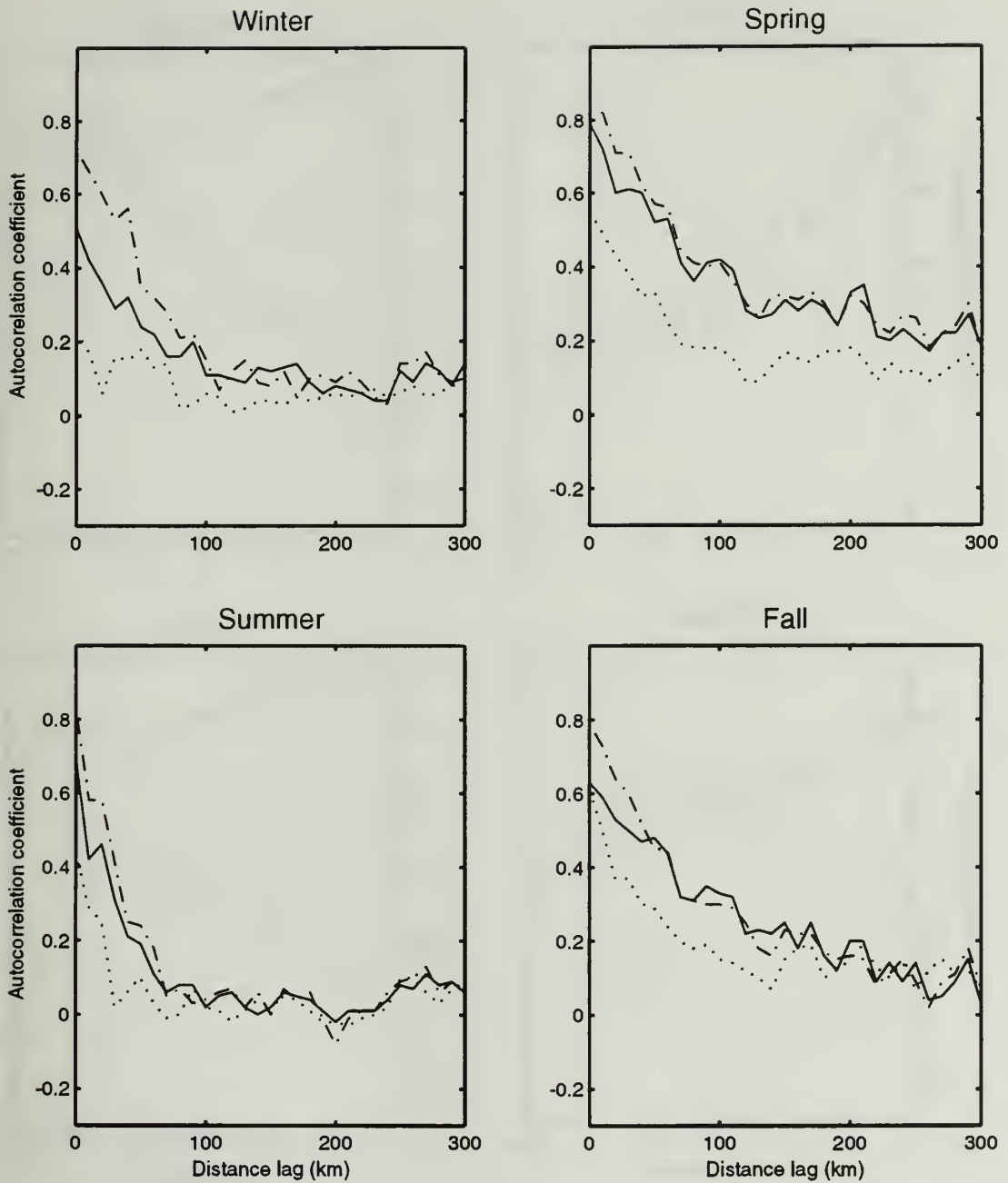
Figure D.9 Spatial Variations of Autocorrelation Function \eta(m, n) for Type II at 80% Water Depth. The Three Curves on Each Graph are the Dependency of \eta(m, n) on Spatial Lag ( m\Delta\gamma ) for n = 0 (no temporal lag, dash-dot), n = 1 (1 day lag, solid), and n = 15 (15 day lag, dots). Data were Obtained from the MOODS Temperature Data Base for the Years 1929 to 1991.
