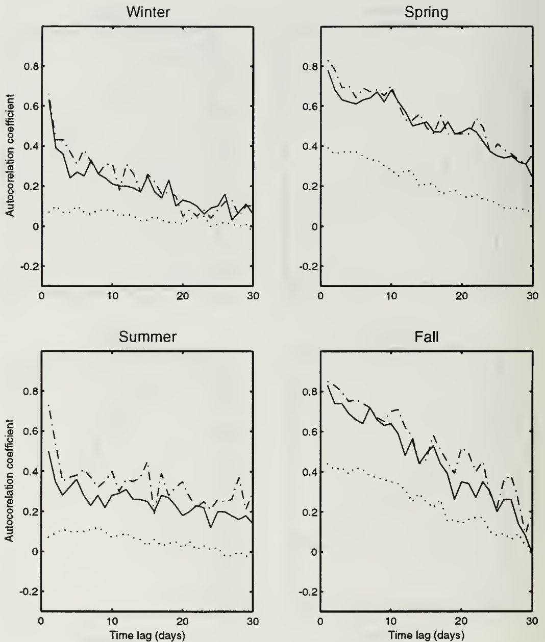
Figure D.2 Temporal Variations of Autocorrelation Function \eta(m, n) for Type II Data at 50% Water Depth. The Three Curves on Each Graph are the Dependency of \eta(m, n) on Time Lag n\Delta t for m = 0 (no lag, dash-dot), m = 1 (10 km lag, solid), and m = 15 (150 km lag, dots). Data were Obtained from the MOODS Temperature Data Base for the Years 1929 to 1991.
