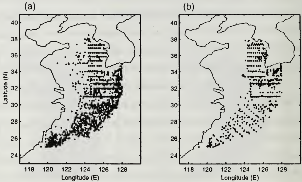
Figure 4.2 (a) Winter Temperature Profile Locations from MOODS Data Base From 1963 to 1977, (b) Locations of Temperature Profiles During Spring 1969, a Period Illustrating Maximum Data Density in a Given Year.
