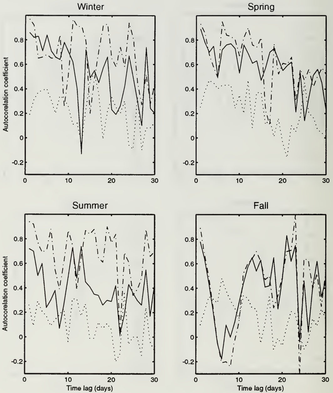
Figure D.6 Temporal Variations of Autocorrelation Function \eta(m, n) for Type III Data at 80% Water Depth. The Three Curves on Each Graph are the Dependency of \eta(m, n) on Time Lag n\Delta t for m = 0 (no lag, dash-dot), m = 1 (10 km lag, solid), and m = 15 (150 km lag, dots). Data were Obtained from the MOODS Temperature Data Base for the Years 1929 to 1991.
