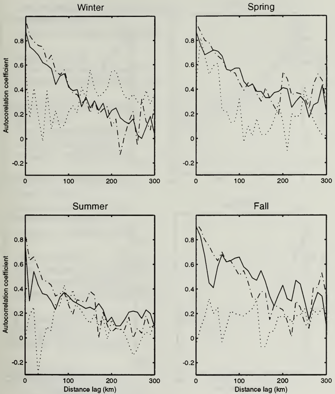
Figure D.11 Spatial Variations of Autocorrelation Function \eta(m, n) for Type III at 50% Water Depth. The Three Curves on Each Graph are the Dependency of \eta(m, n) on Spatial Lag ( m\Delta\gamma ) for n = 0 (no temporal lag, dash-dot), n = 1 (1 day lag, solid), and n = 15 (15 day lag, dots). Data were Obtained from the MOODS Temperature Data Base for the Years 1929 to 1991.
