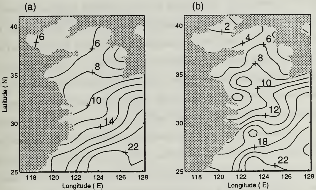
Figure 4.6 Climatological SST Field on (a) a 30 Minute Grid and (b) a 20 Minute Grid.
