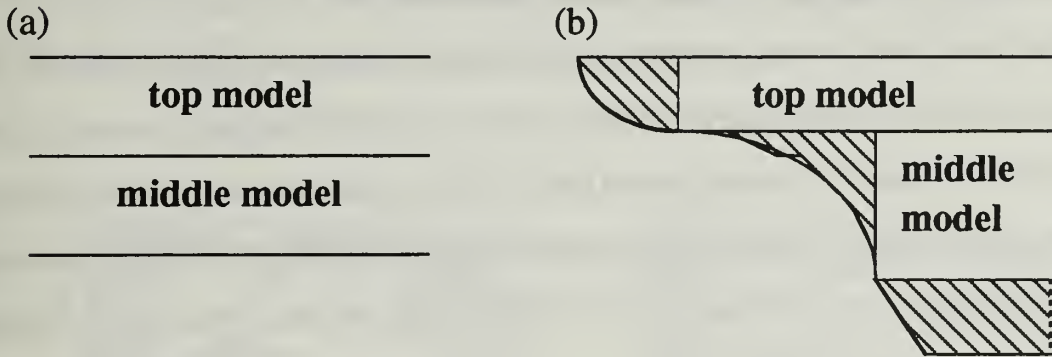
Figure 4.4 The Geometries of Vertical Submodel in the Construction of Climatology Temperature Profiles in the (a) Deep Water and (b) Continental Shelf.
