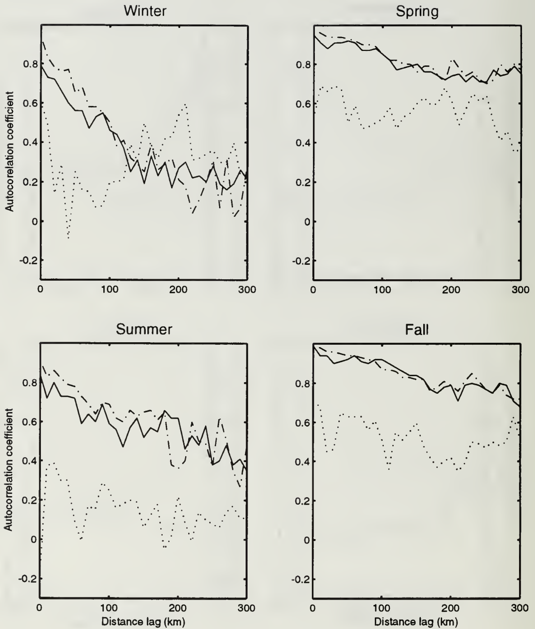
Figure D.10 Spatial Variations of Autocorrelation Function \eta(m, n) for Type III at the Surface. The Three Curves on Each Graph are the Dependency of \eta(m, n) on Spatial Lag ( m\Delta\gamma ) for n = 0 (no temporal lag, dash-dot), n = 1 (1 day lag, solid), and n = 15 (15 day lag, dots). Data were Obtained from the MOODS Temperature Data Base for the Years 1929 to 1991.
