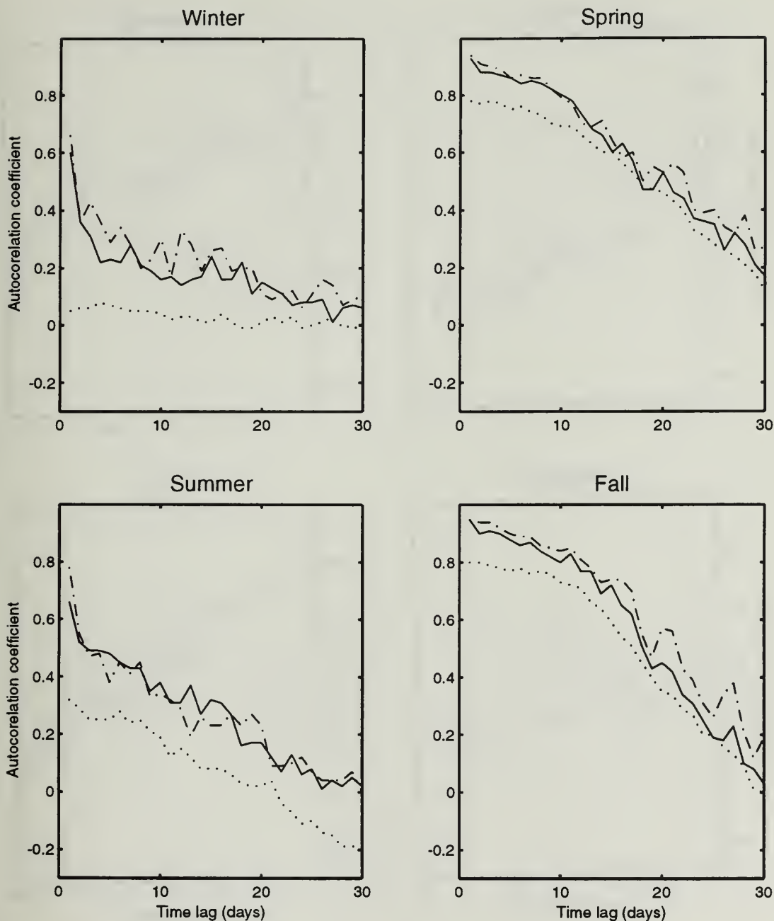
Figure D.1 Temporal Variations of Autocorrelation Function \eta(m, n) for Type II Data at the Surface. The Three Curves on Each Graph are the Dependency of \eta(m, n) on Time Lag n\Delta t for m = 0 (no lag, dash-dot), m = 1 (10 km lag, solid), and m = 15 (150 km lag, dots). Data were Obtained from the MOODS Temperature Data Base for the Years 1929 to 1991.
