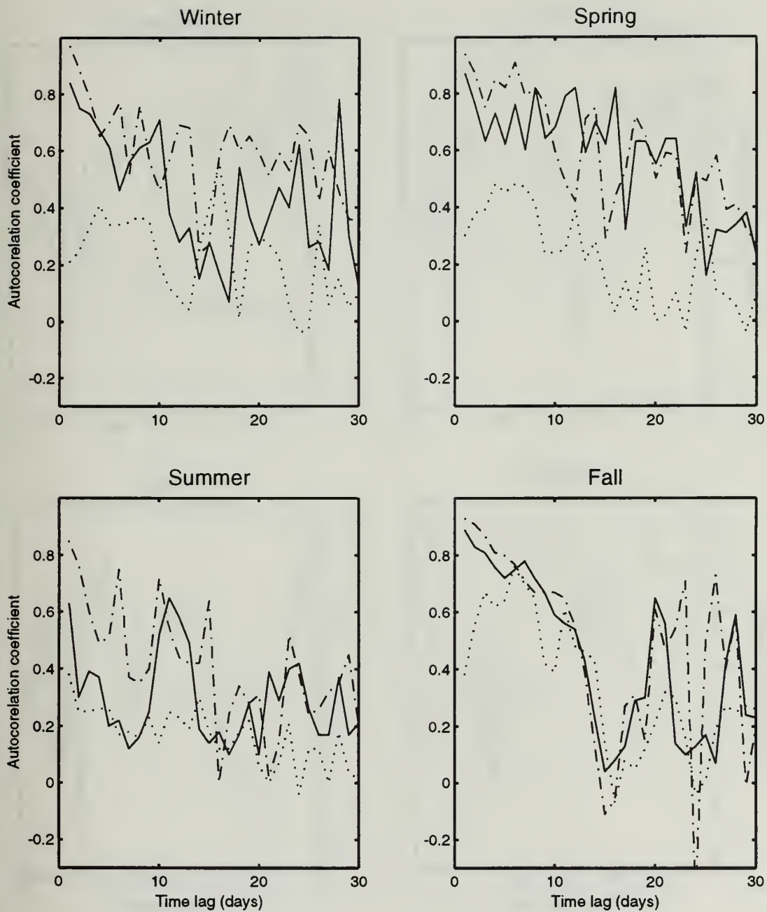
Figure D.5 Temporal Variations of Autocorrelation Function \eta(m, n) for Type III Data at 50% Water Depth. The Three Curves on Each Graph are the Dependency of \eta(m, n) on Time Lag n\Delta t for m = 0 (no lag, dash-dot), m = 1 (10 km lag, solid), and m = 15 (150 km lag, dots). Data were Obtained from the MOODS Temperature Data Base for the Years 1929 to 1991.
