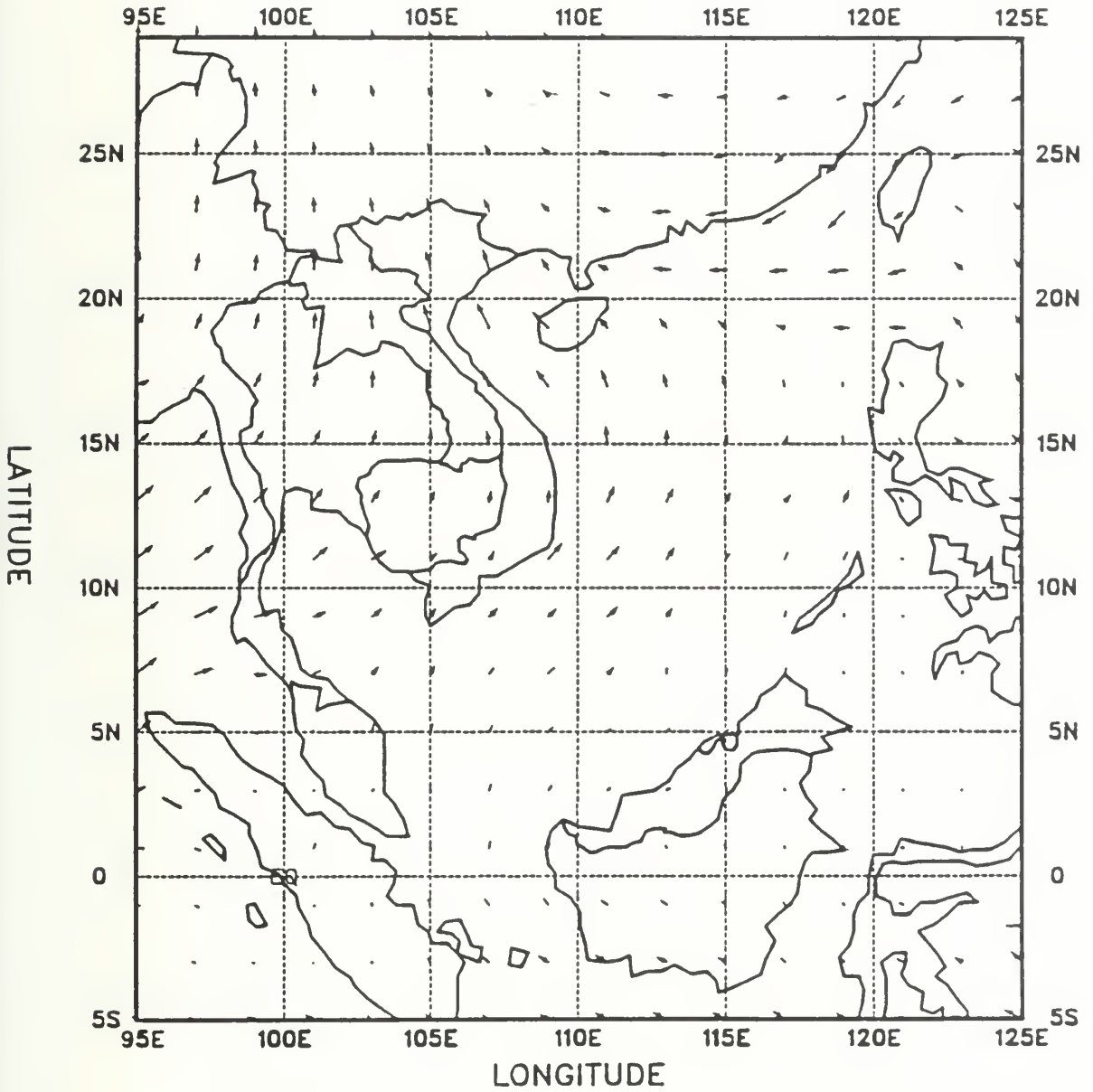
Figure 14A : Summer (May) Hellerman Wind Stress Distribution
