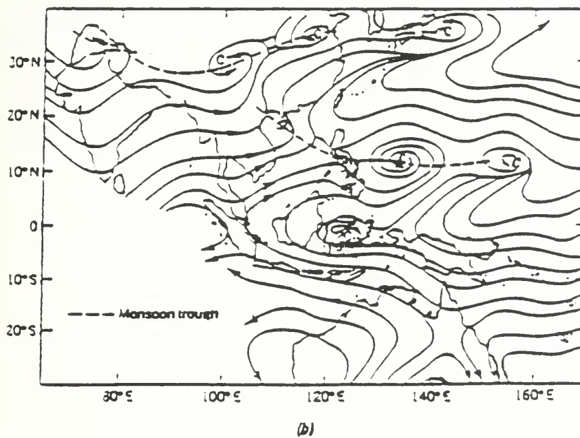
Figure 6 : The Mean 850-mb Streamline of the Southeast Asia Monsoons (a) December, (b) July (Cheang, 1987)
