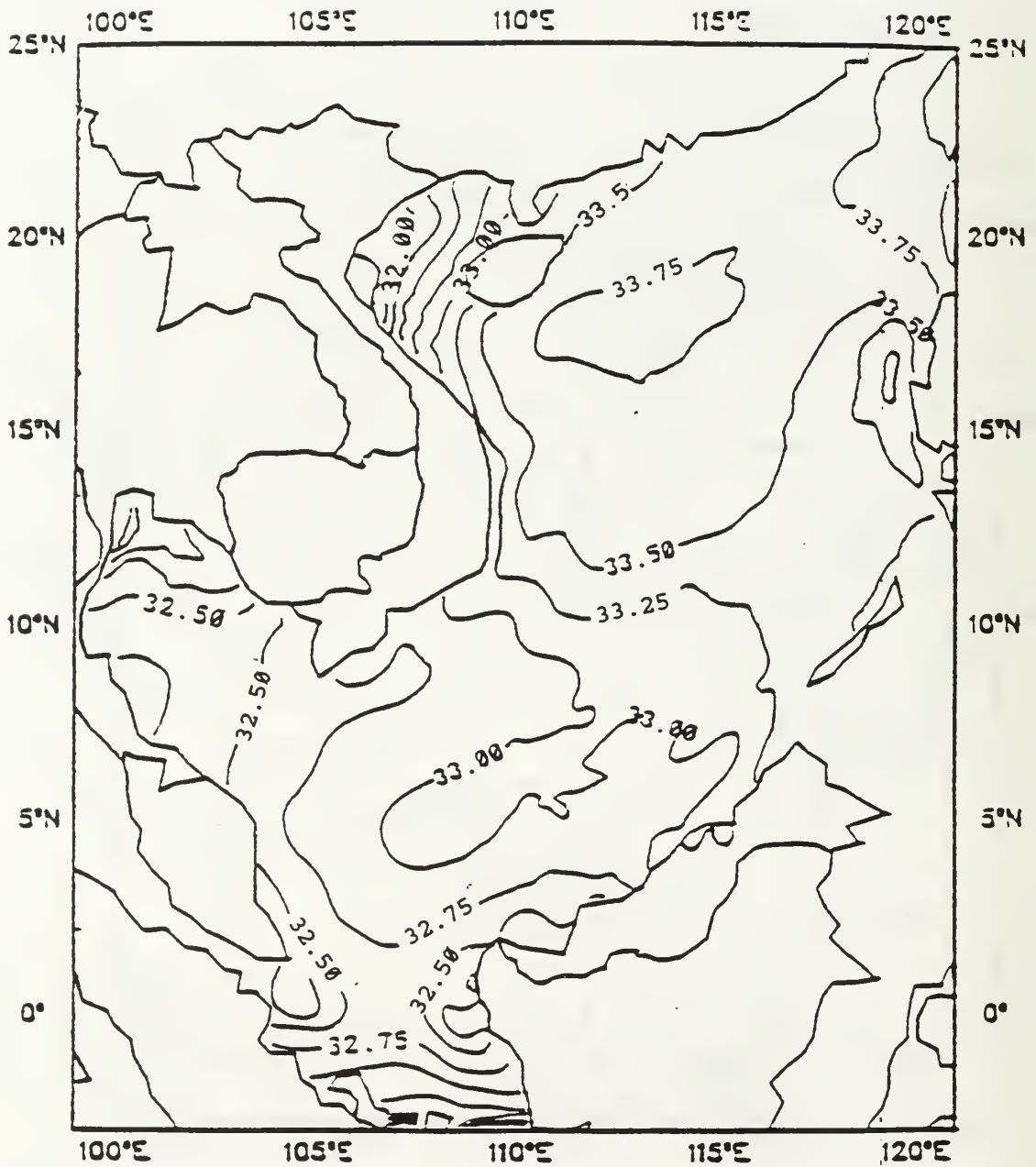
Figure 17B :Simulated Winter (10 December) Surface Salinity (psu) Distribution;
