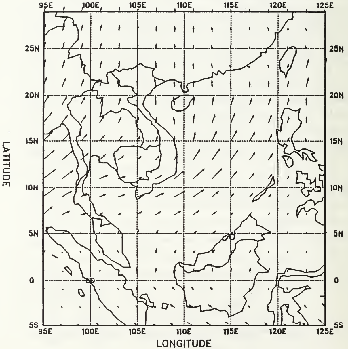
Figure 14B : Summer (June) Hellerman Wind Stress Distribution
