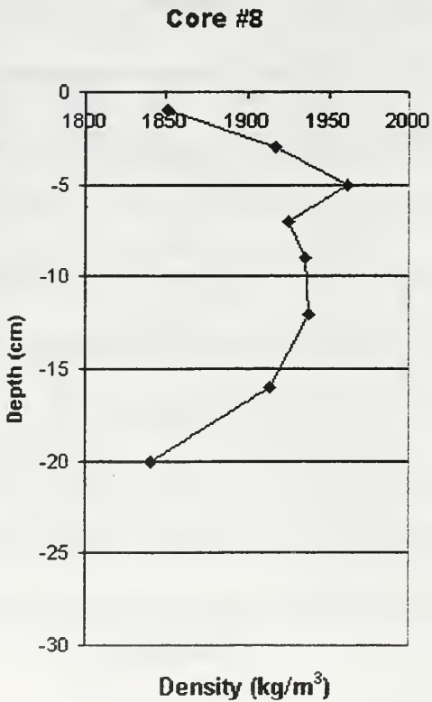
Figure 12. Density Vs. Depth for Cores 6-9.
