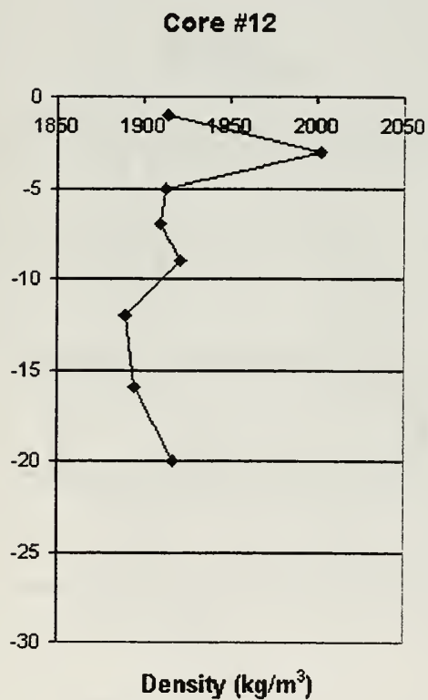
Figure 13. Density Vs. Depth for Cores 10-12.
