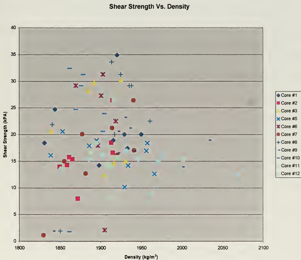
Figure 17. Shear Strength Vs. Density analyzed on June 1, 2000.
