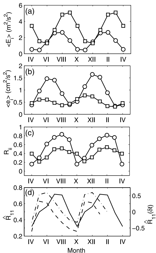
Figure 13. Characteristics of the annual oscillation in the eastern subbasin: (a) the mean wind KE, (b) the mean KE of mid-depth currents, (c) correlations between wind stress and currents, and (d) correlations between the wind stress curl and the stream function of mid-depth currents. Here circles and squares represent zonal and meridional components. Solid, dotted-dashed, and dashed curves in Figure 13d correspond to 0-, 2- and 3-month lags, respectively.
