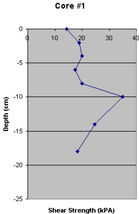
Fig. 5 Sediment shear strength profile at the gravity core #1.
