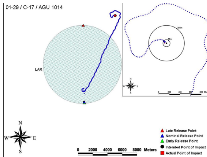
Figure 6. Typical 10K Screamer trajectory (top view) with JPADS-MP LAR computation shown and insert of final approach to the PI
