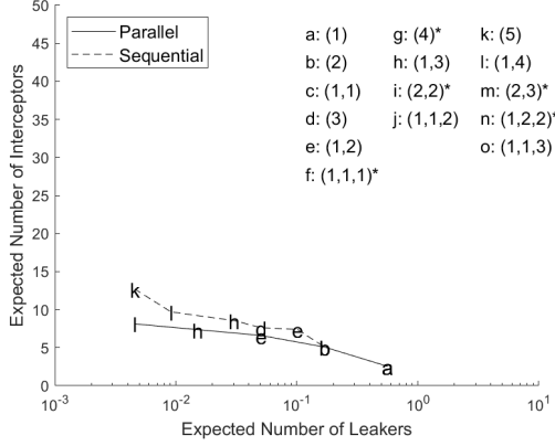
(a) Good SM per-round kill probability ( \theta_1 = 0.5 ) and Good false-negative probability ( \gamma_0 = 0.3 )
