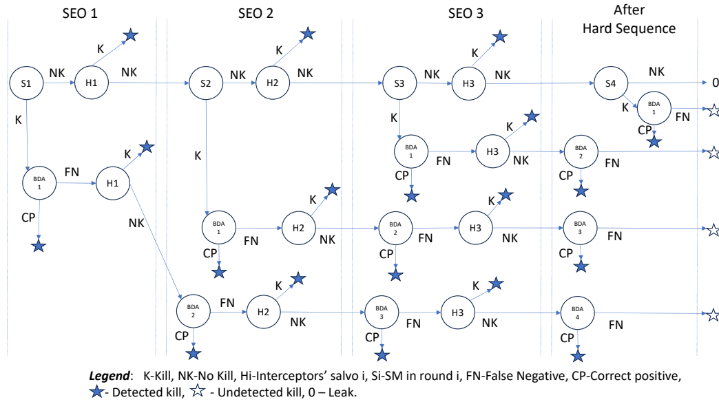
Figure 1 Event tree describing the engagement of one threat for K = 3 SEOs. Note that SM can be active both prior to the initiation of the HD sequence (S1 occurs before H1) and after the HD sequence concludes (S4 occurs after H3).
