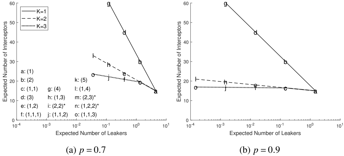
Figure 2 Efficient Frontier in Expected Number of Interceptors vs Expected Number of Leakers space for various values of K and p . x-axis is on a log scale. In the legend, sequences are marked with an asterisk (*) if they are inefficient for all combinations of K and p .
