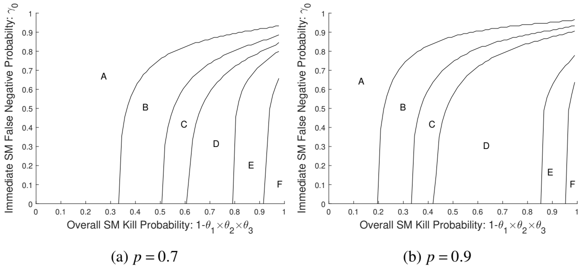
Figure 4 Efficient Frontier Regions for K = 3 and N \in \{1, 2, 3, 4, 5\} for different SM false-negative and SM kill probability combinations. In each region the efficient frontier is the same. See the text for the efficient frontier corresponding to each region
