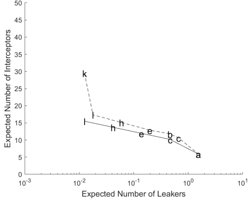
(c) Moderate SM per-round kill probability ( \theta_1 = 0.7 ) and Good false-negative probability ( \gamma_0 = 0.3 )
