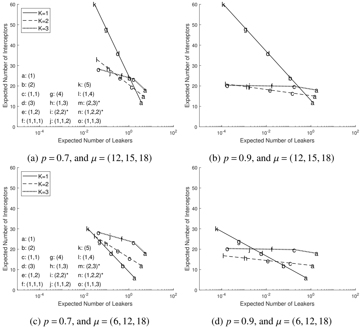
Figure 3 Expected Number of Interceptors vs Expected Number of Leakers when Blue has K SEOs against W_K threats. x-axis is on a log scale. In the legend, sequences are marked with an asterisk (*) if they are inefficient for all combinations of K and p .
