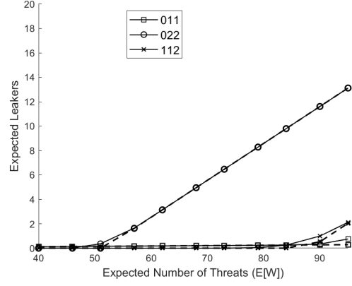
(b) Expected Number of Leakers, p = 0.9
