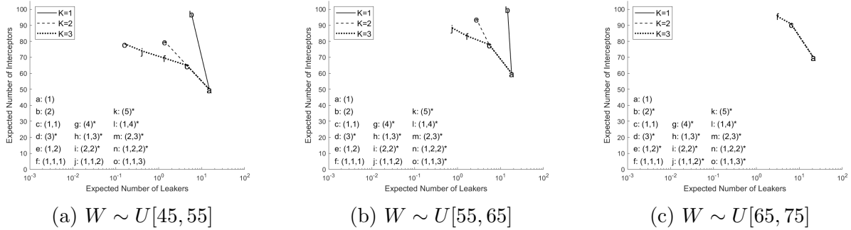
Figure 8: Efficient Frontier in Expected Number of Interceptors vs Expected Number of Leakers space for p = 0.7 and various values of K and \mathbf{E}[W] . x-axis is on a log scale. In the legend, sequences are marked with an asterisk (*) if they are inefficient for all values of K .
