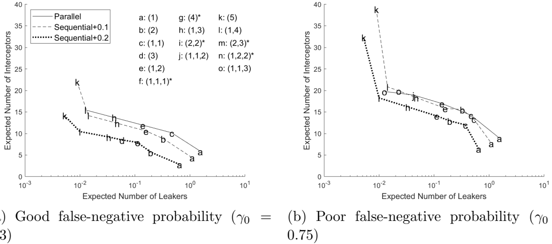
Figure 10: Parallel SM and Improved Sequential SM. Expected Number of Interceptors vs Expected Number of Leakers for p = 0.7 , W \sim U[10, 20] , Moderate Parallel SM per-round kill probability ( \theta_1^{(\text{parallel})} = 0.7 ), and \gamma_0 \in \{0.3, 0.75\} . x-axis is on a log scale. In the legend, sequences are marked with an asterisk (*) if they are inefficient for all scenarios across the two figures.
