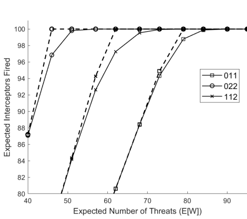
(c) Expected Number of Interceptors, p = 0.7
