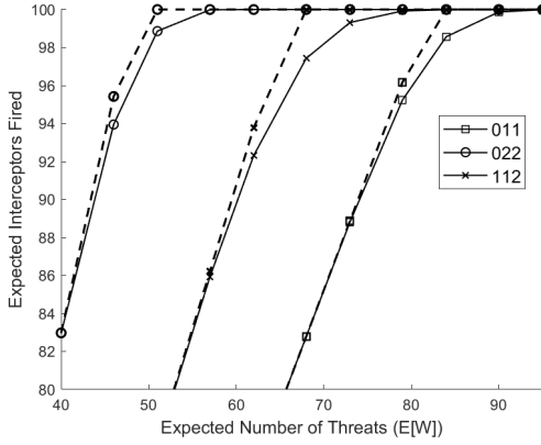
(c) Expected Number of Interceptors, p = 0.7
