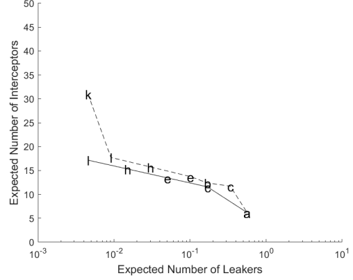
(b) Good SM per-round kill probability ( \theta_1 = 0.5 ) and Poor false-negative probability ( \gamma_0 = 0.75 )
