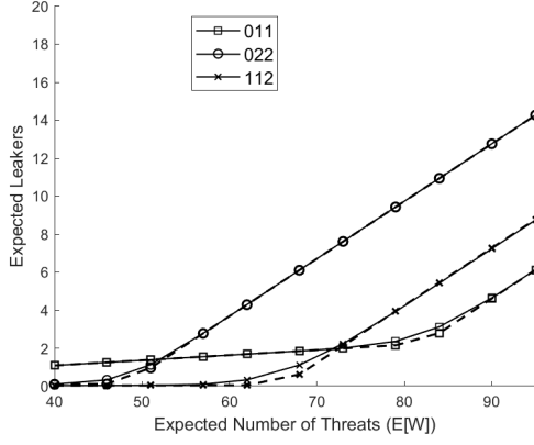
(a) Expected Number of Leakers, p = 0.7
