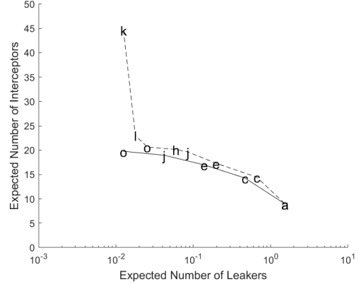
(d) Moderate SM per-round kill probability ( \theta_1 = 0.7 ) and Poor false-negative probability ( \gamma_0 = 0.75 )
