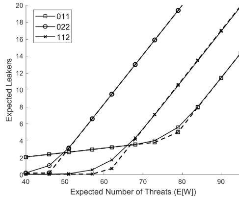
(a) Expected Number of Leakers, p = 0.7
