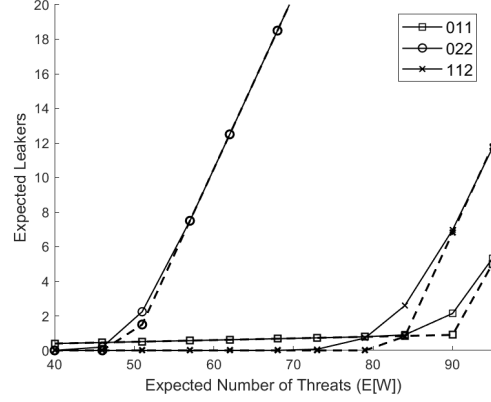
(b) Expected Number of Leakers, p = 0.9
