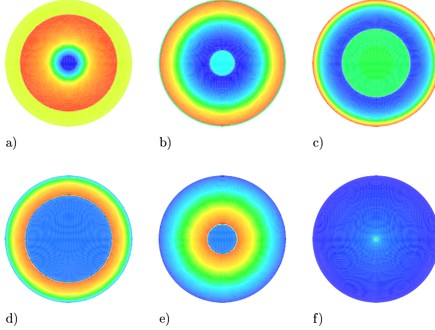
FIG. 11. Case 5. Color contours of \phi (left), u_s (center), and v_s (right) for the DG strong conservation form with O(2N) integration for the resolution n_I = 64 and N = 1 at a) 1 day, b) 2 days, c) 3 days, d) 4 days, e) 5 days, and f) 5.4 days. Figures a, b, and c are viewed from (\lambda, \theta) = (180, 0) and d, e, and f from (\lambda, \theta) = (0, 0) .
