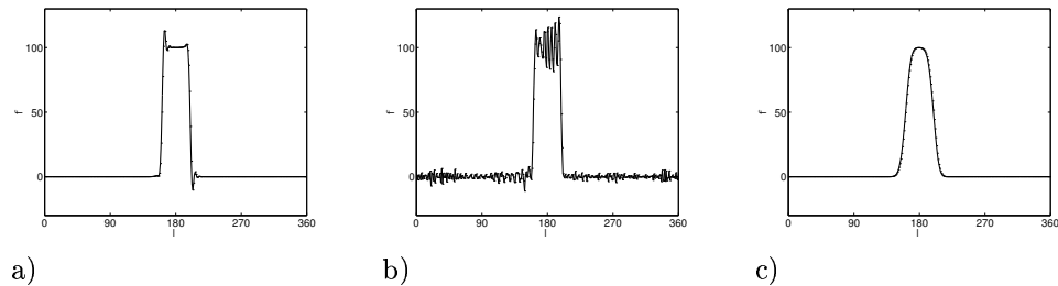
FIG. 9. Case 4. Profile of the geopotential height, \phi , along the Equator after 12 days for n_I = 64 and N = 1 for the a) DG strong conservation form with O(2N) integration, b) spectral element, and c) the DG0 method.
