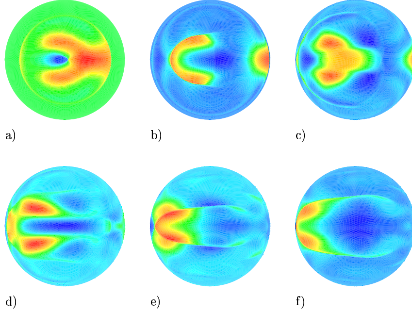
FIG. 12. Case 6. Color contours of \phi (left), u_s (center), and v_s (right) for the DG strong conservation form with O(2N) integration for the resolution n_I = 64 and N = 1 at a) 1 day, b) 2 days, c) 3 days, d) 4 days, e) 5 days, and f) 5.4 days. All the figures are viewed from (\lambda, \theta) = (180, 0) .
