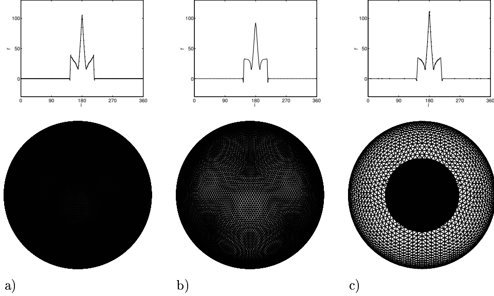
FIG. 13. Case 7. Profile of the geopotential height, \phi , along the Equator and corresponding grid after 0.5 days for the DG strong conservation with O(2N) integration on a) icosahedral grid with 40,962 grid points ( n_I = 64 ), b) icosahedral grid with 16,002 grid points ( n_I = 40 ), and c) adaptive grid with 15,695 grid points.
