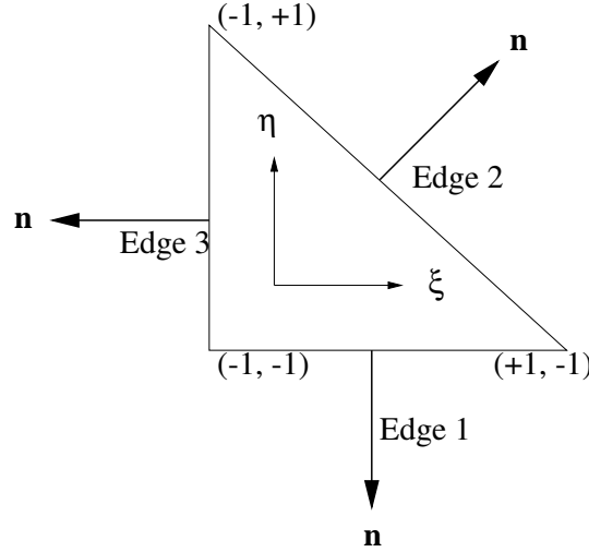
FIG. 2. The normal vectors of the master triangle.
