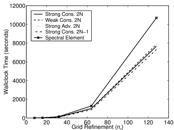
FIG. 14. The wallclock time required to perform a one day integration as a function of grid refinement level, n_I , using N = 1 for the strong conservation form with O(2N) integration (solid line), weak conservation form with O(2N) integration (dashed line), strong advection form with O(2N) integration (dotted line), strong conservation form with O(2N - 1) integration (dash-dotted line), and the spectral element method (solid line with square).
