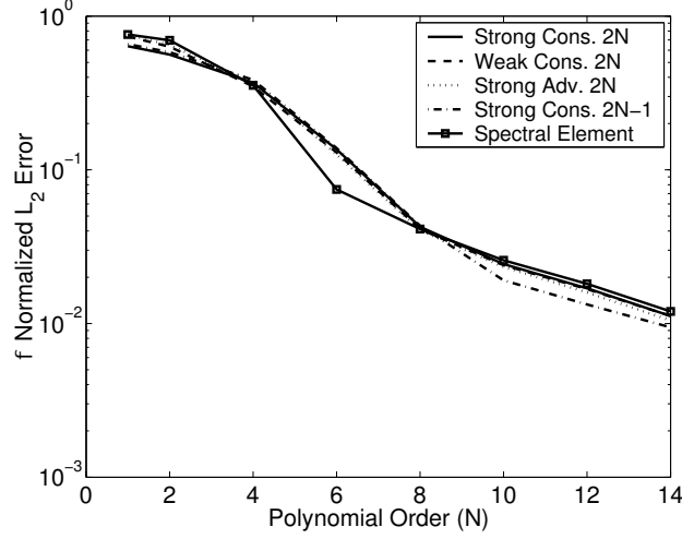
FIG. 5. Case 1. The normalized \phi L_2 error as a function of polynomial order, N , after 12 days using 80 ( n_I = 2 ) elements for the strong conservation form with O(2N) integration (solid line), weak conservation form with O(2N) integration (dashed line), strong advection form with O(2N) integration (dotted line), strong conservation form with O(2N - 1) integration (dashed-dotted line), and the spectral element method (solid line with square).
