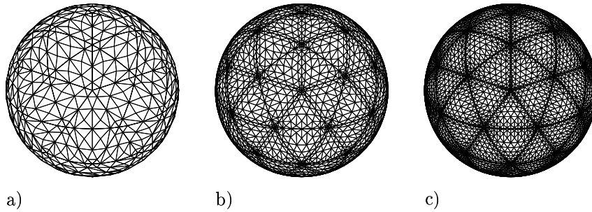
FIG. 4. Icosahedral grid for n_I = 2 and a) N = 4 , b) N = 8 , and c) N = 12 .
