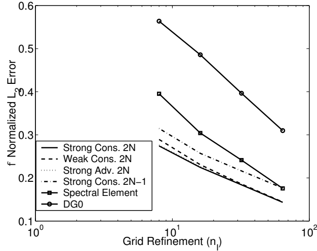
FIG. 8. Case 4. The normalized \phi L_2 error as a function of grid refinement, n_I , after 12 days using N = 1 order elements for the strong conservation form with O(2N) integration (solid line), weak conservation form with O(2N) integration (dashed line), strong advection form with O(2N) integration (dotted line), strong conservation form with O(2N - 1) integration (dashed-dotted line), spectral element method (solid line with square), and the DG0 method (solid line with circle).
