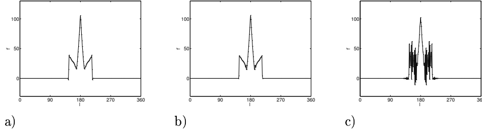
FIG. 10. Case 5. Profile of the geopotential height, \phi , along the Equator after 0.5 days for n_I = 64 and N = 1 for the a) conservation forms, b) strong advection form, and c) spectral element method.
