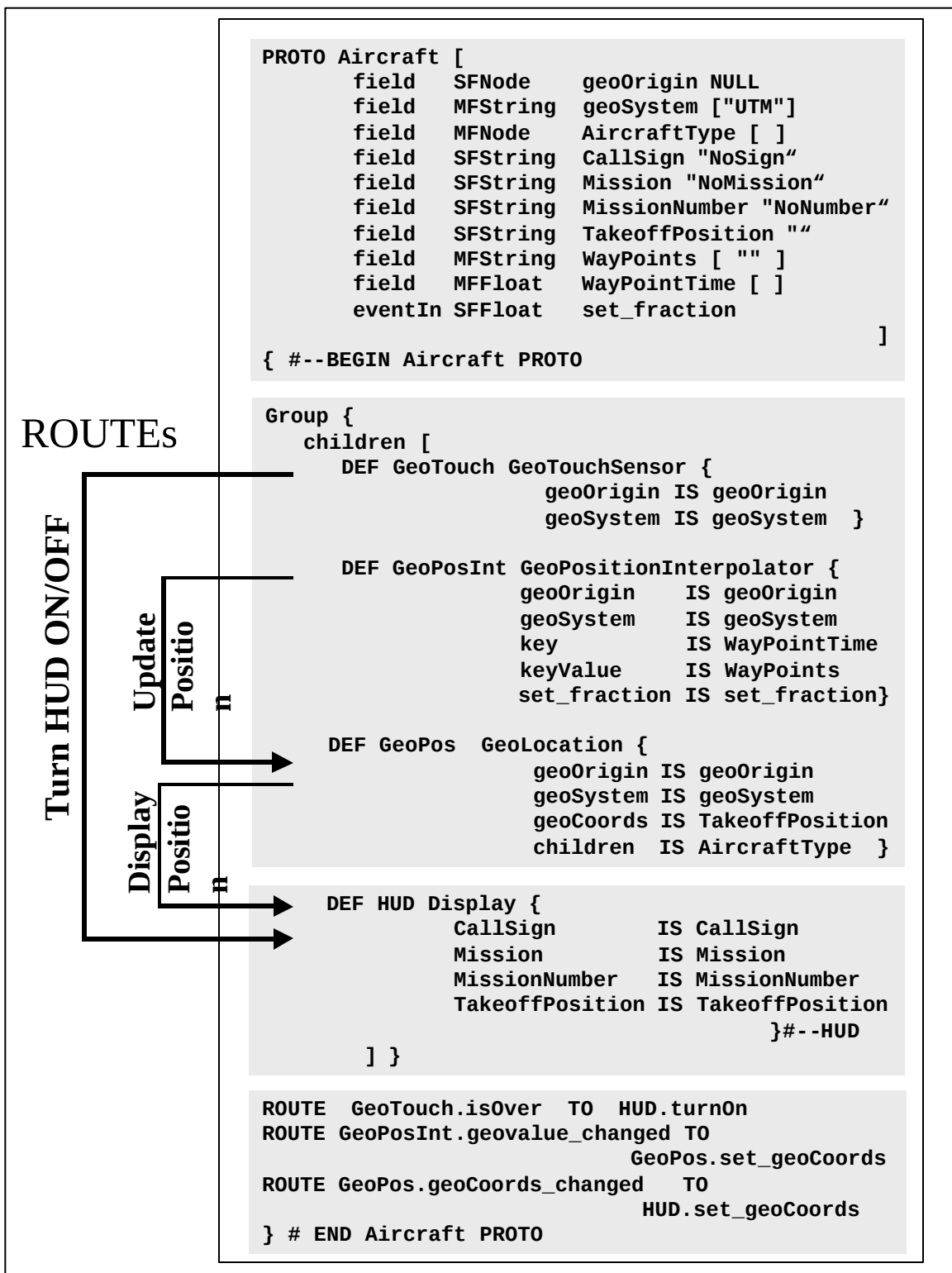
Figure 7.4. Aircraft PROTO with ROUTE wiring for event passing
