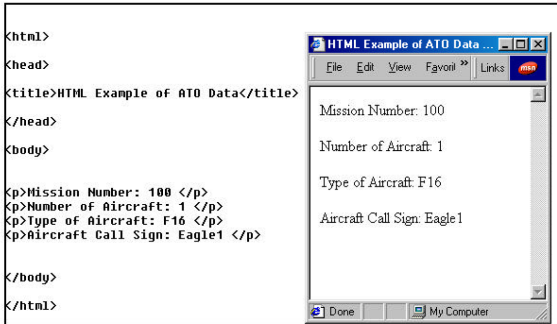
Figure 2.1. HTML Example
