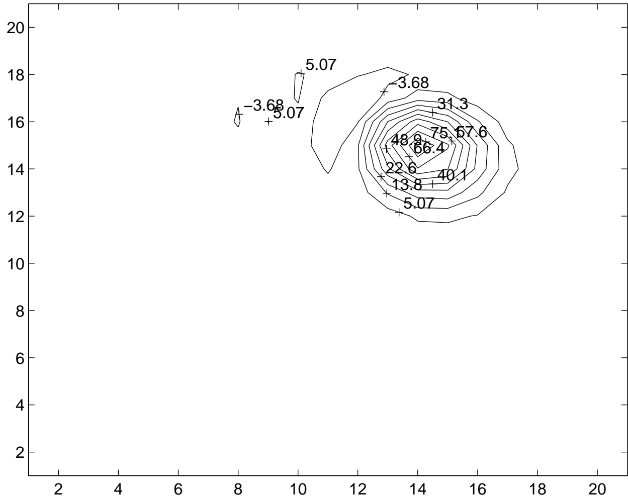
concentration after 0.375 revolutions
