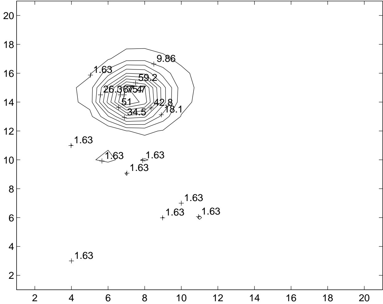
concentration after 0.125 revolutions
