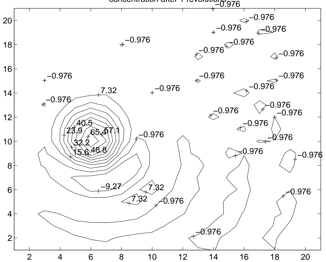
concentration after 1 revolutions
