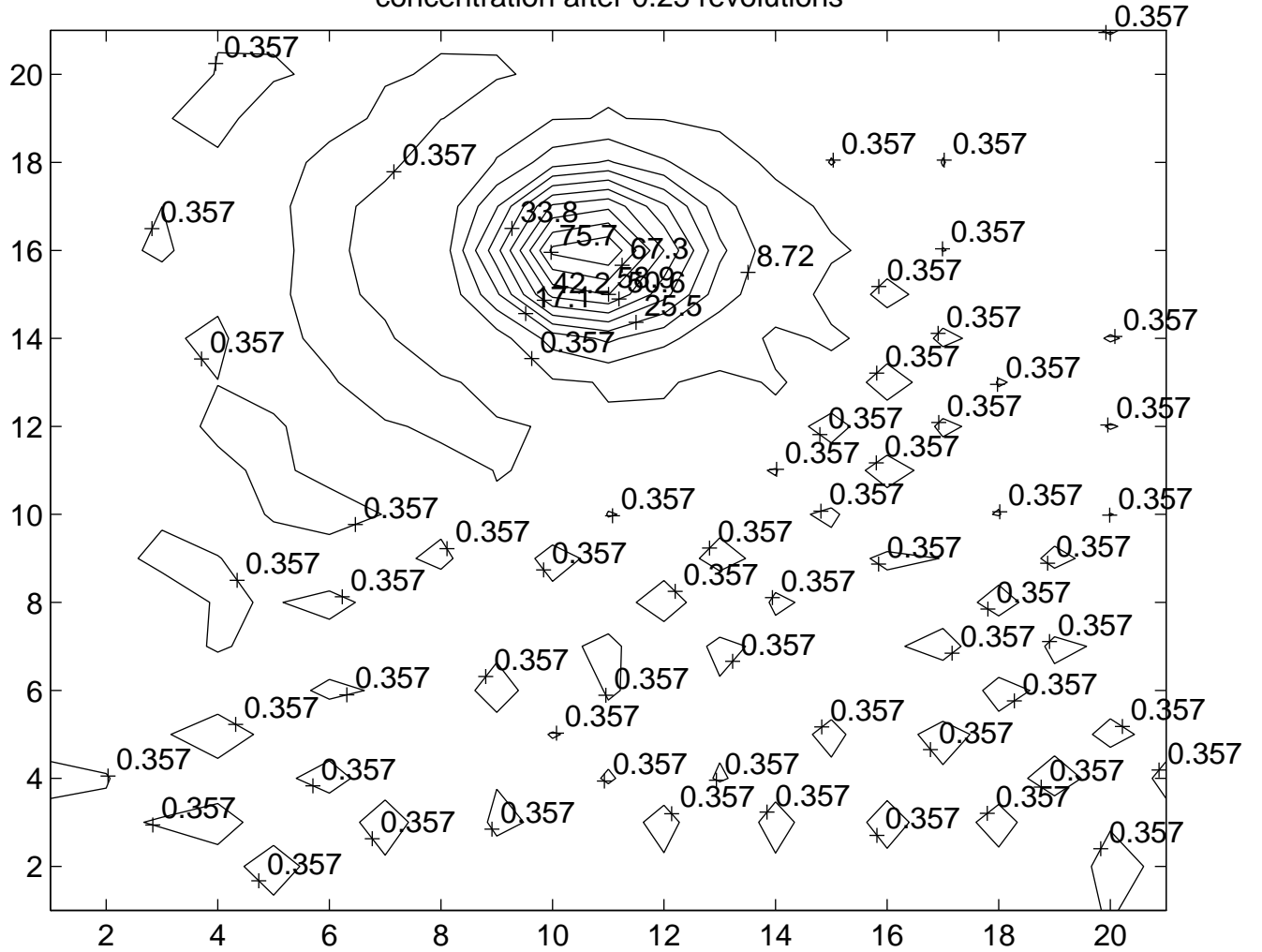
concentration after 0.25 revolutions
