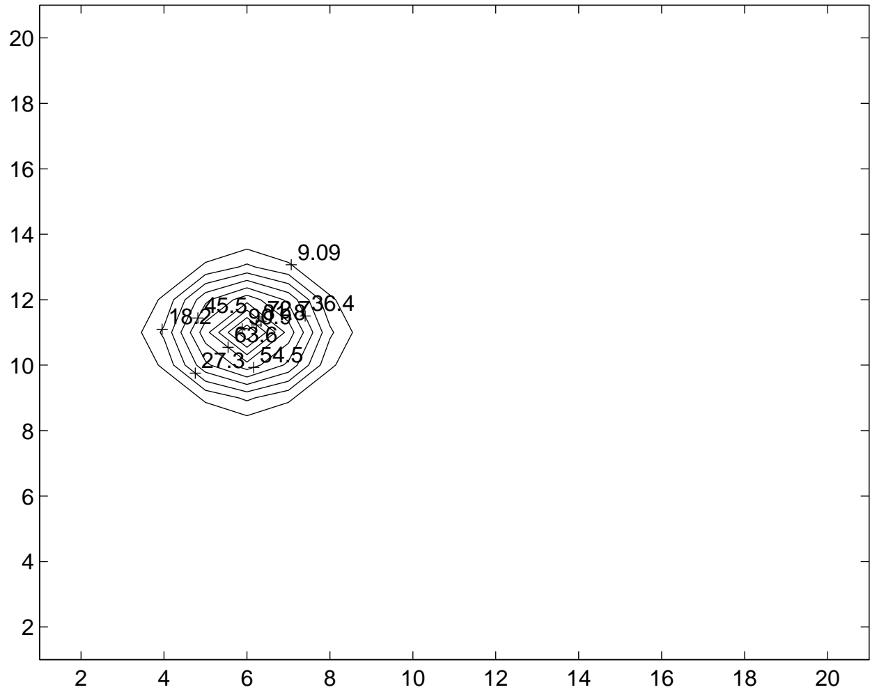
concentration after 0 revolutions
