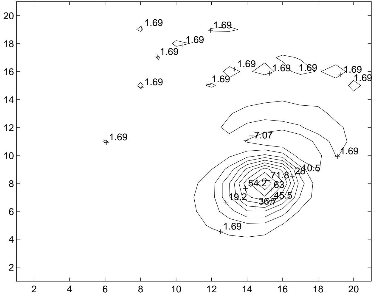
concentration after 0.625 revolutions
