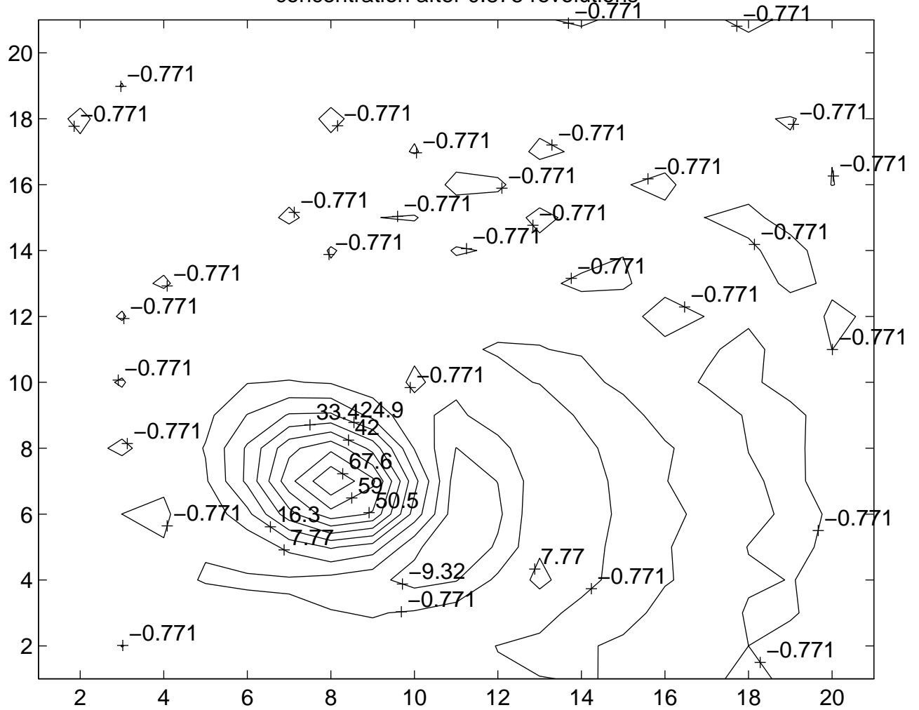
concentration after 0.875 revolutions
