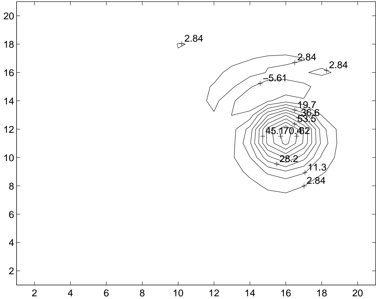
concentration after 0.5 revolutions
