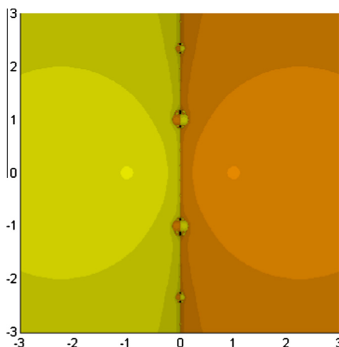
Fig. 1. Our method with c = -3.53 for the roots of the polynomial z^2 - 1 .
