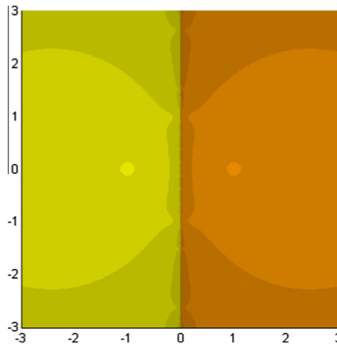
Fig. 2. Our method with c = -3 for the roots of the polynomial z^2 - 1 .
