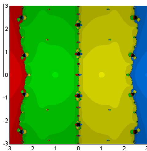
Fig. 10. Our method with c = -3 for the roots of the polynomial z^4 - 10z^2 + 9 .
