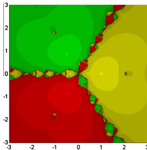
Fig. 8. Our method with c = -1.125 for the roots of the polynomial z^3 - 1 .
