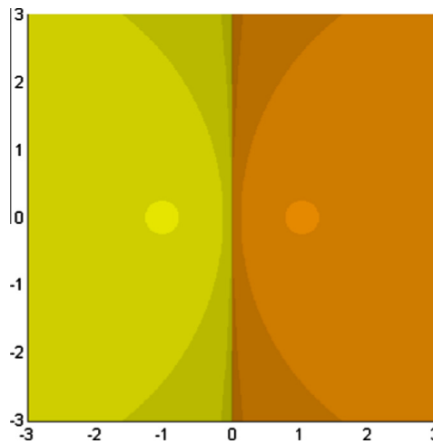
Fig. 3. Kou-Li's method with c = -9/4 for the roots of the polynomial z^2 - 1 .
