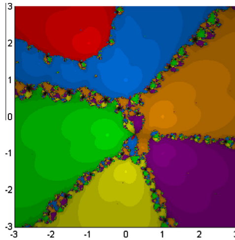
Fig. 20. Our method with c = -1.125 for the fifth example.
