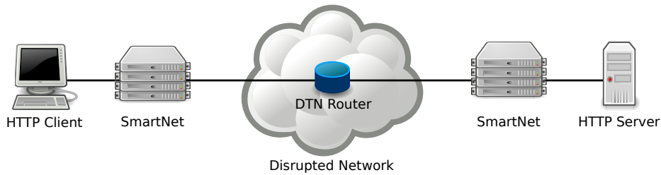
Figure 5.1: DTN-enabled network used to test the SmartNet performance. HTTP performance was tested over a disrupted network traversing two DTN hops with a variety of SmartNet configurations.
