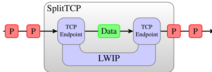
Figure 4.4: SplitTCP plugin operation. The SplitTCP plugin creates two new TCP endpoints. When packets arrive the data is read from one endpoint and sent out from the other endpoint using the LWIP TCP/IP stack.
