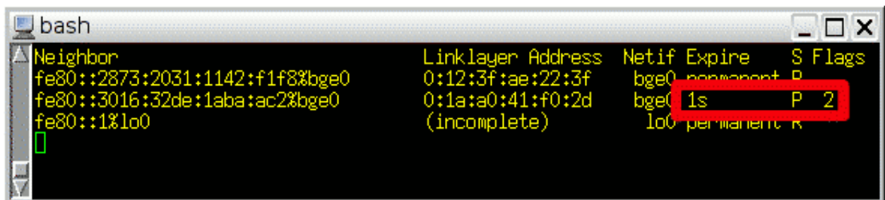
Figure 25. Second stage—PROBE state assigned to Victim's entry.
