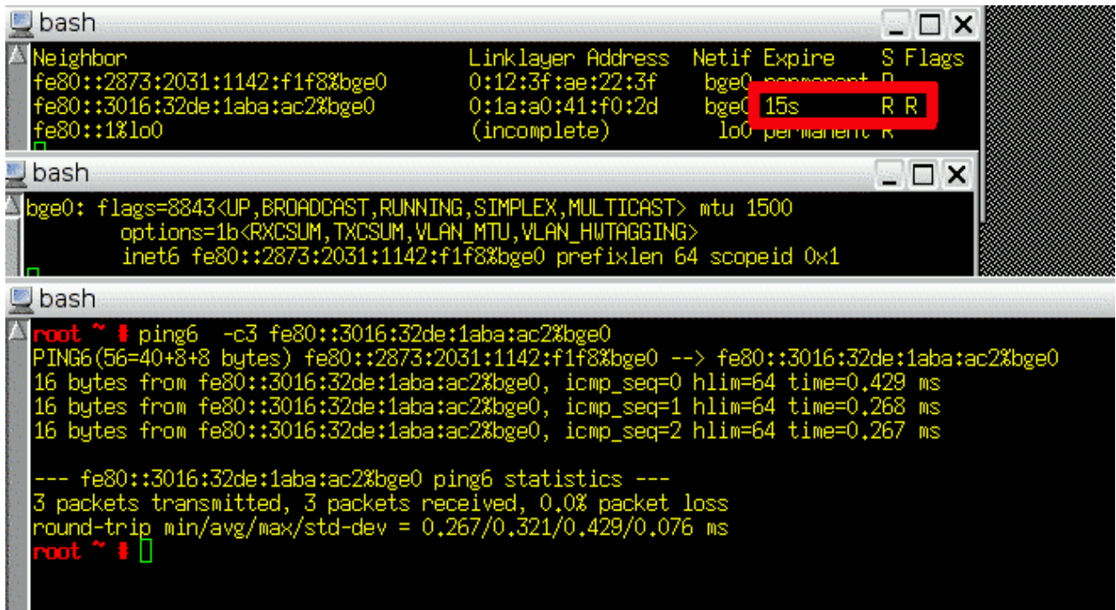
Figure 12. Monitoring setup on the Client.
