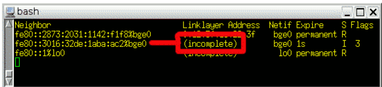
Figure 26. Third stage—INCOMPLETE state assigned to Victim's entry.
