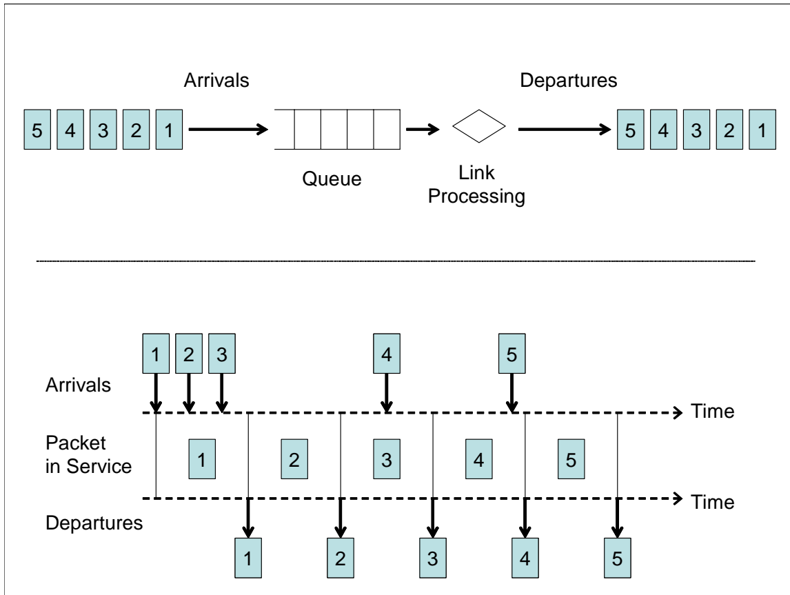
Figure 5. FIFO Queuing.
