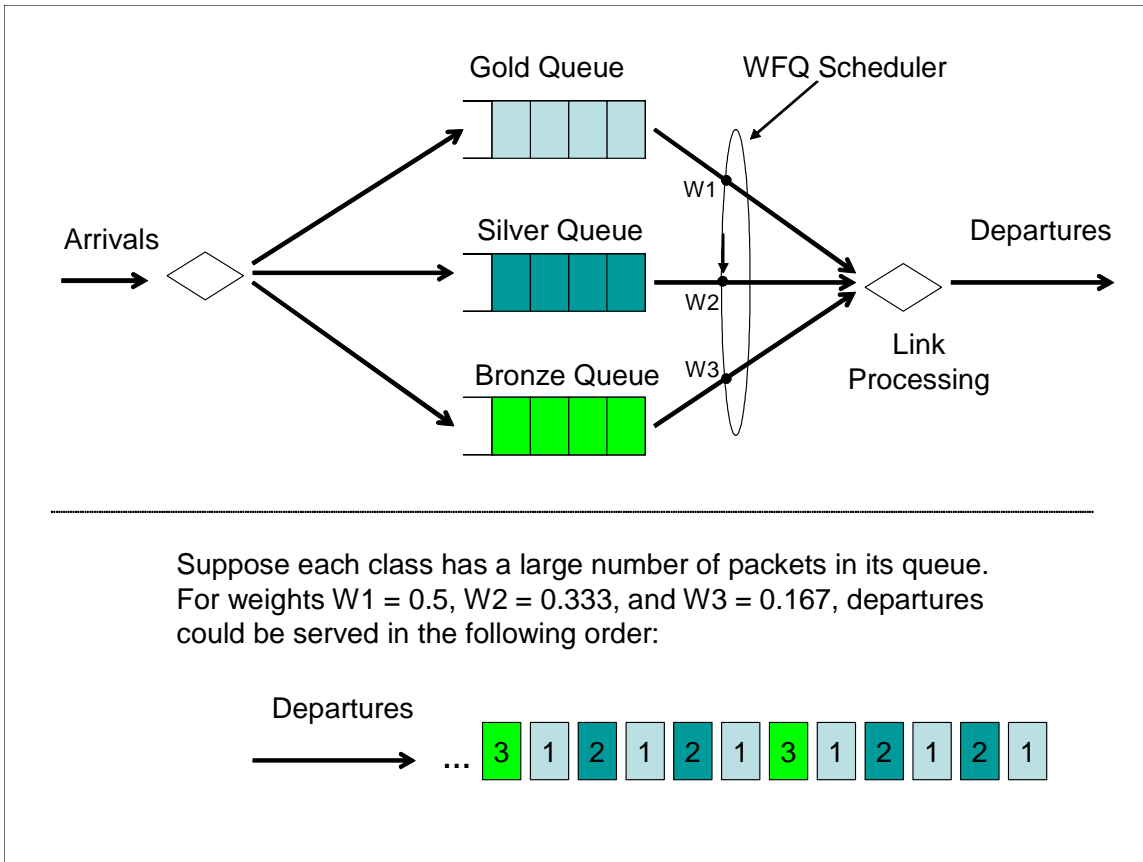
Figure 8. WFQ Scheduling.
