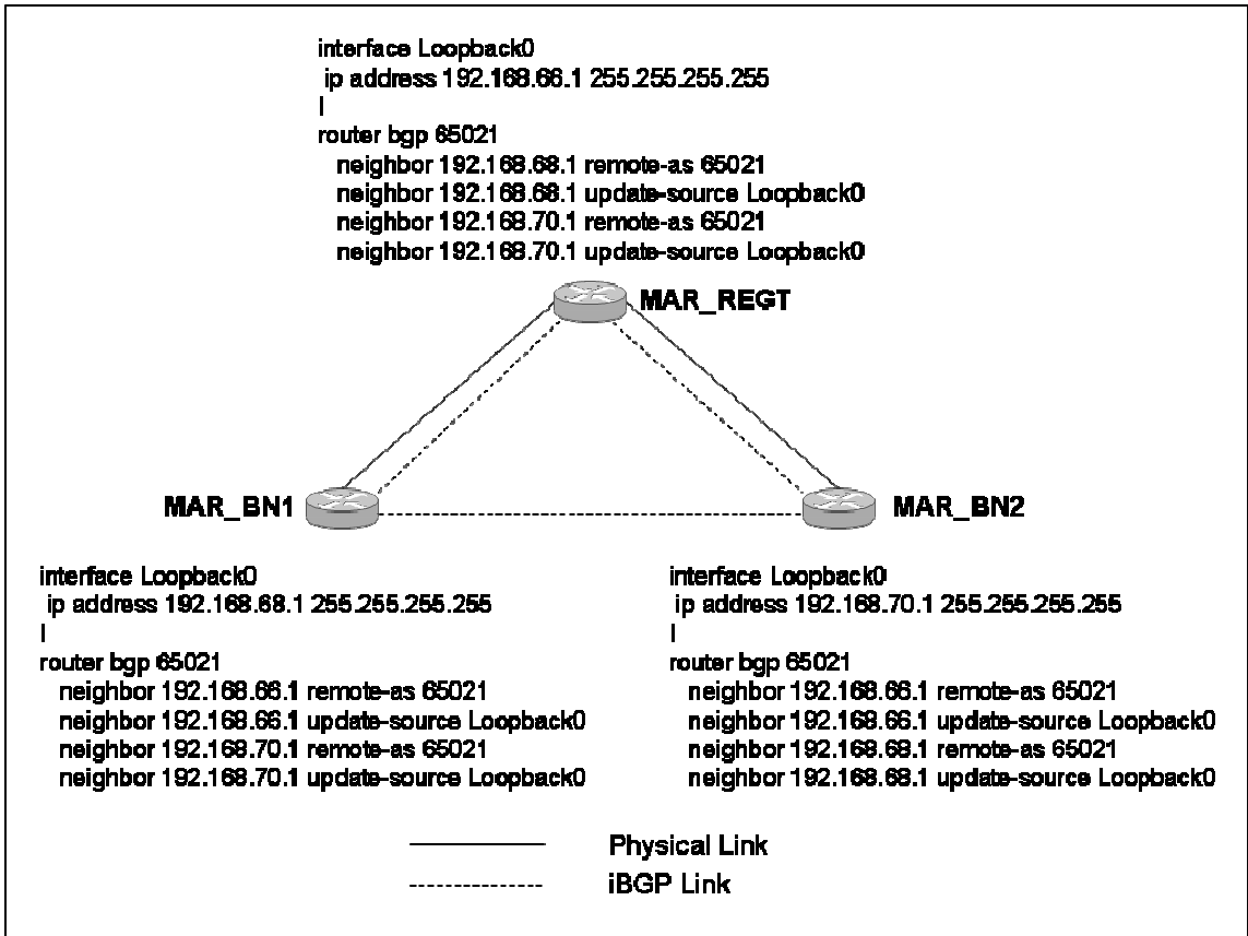
Figure 14. iBGP Configuration.
