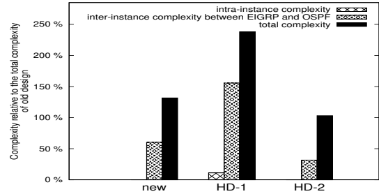
Figure 13: Comparison of complexity of different designs.
