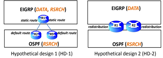
Figure 12: The two hypothetical designs.
