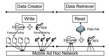
Fig. 2. Existing MDFS architecture
