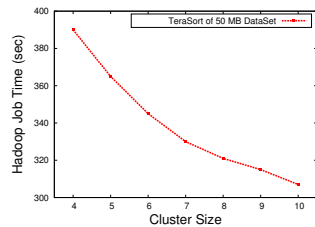
Fig. 6. Effect of Cluster size on Job Completion Time
