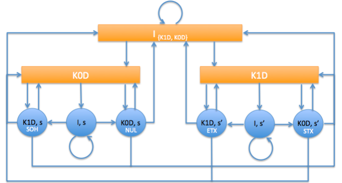
Fig. 5. 2-bit ASCII decoder
