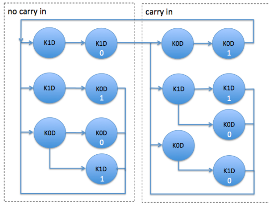
Fig. 6. Incremental ripple-carry-addder
