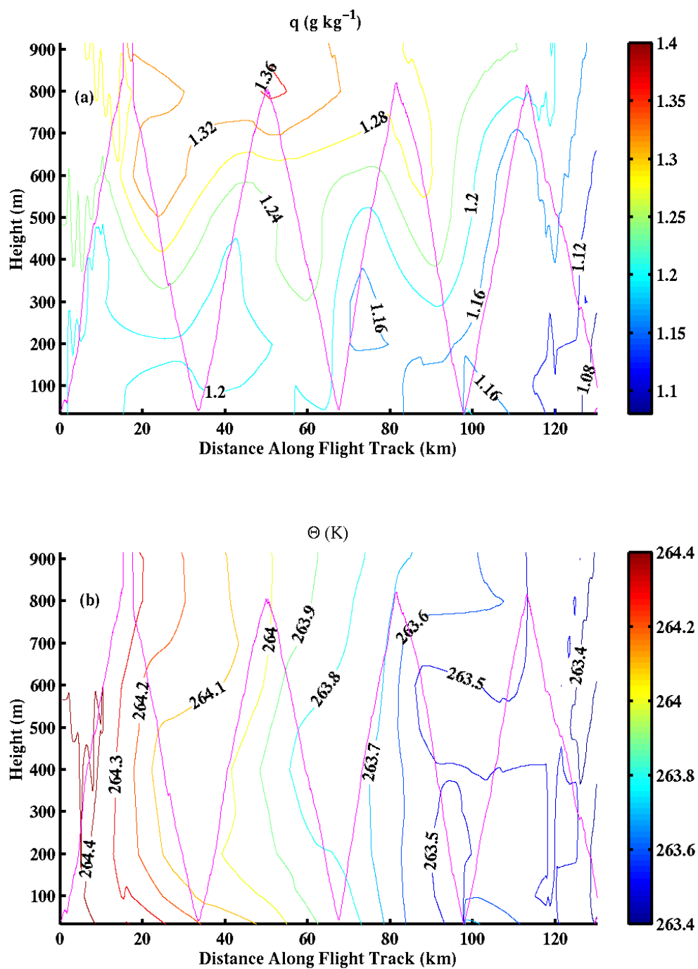
Figure 4.10. BL cross-sections in the up-wind direction (along the flight track) of (a) water vapor ( \text{g kg}^{-1} ) and (b) potential temperature (K) derived from eight sounding legs. The sounding flight track is shown within the contour plots. See Figure 4.7 for the locations of the soundings.
