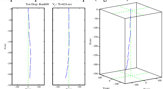
Figure 23. Model bomb tracks obtained using MATLAB.
