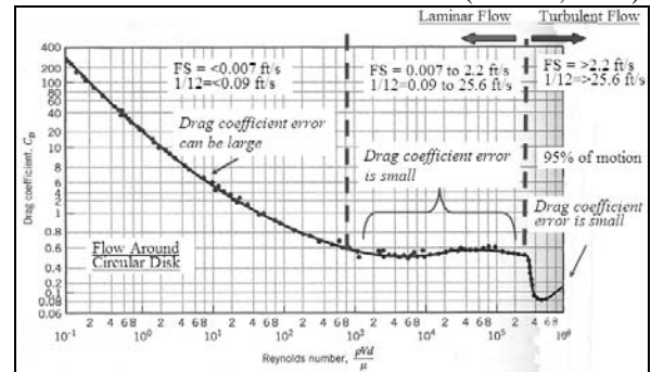
Figure 6. Drag coefficient versus Reynolds number (From: Gefken, 2005)
