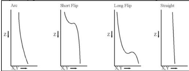
Figure 25. Generalized trajectory patterns.
