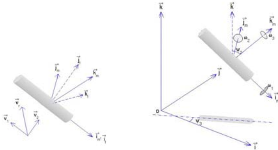
Figure 5. Three coordinate systems (from Chu et al., 2004).
