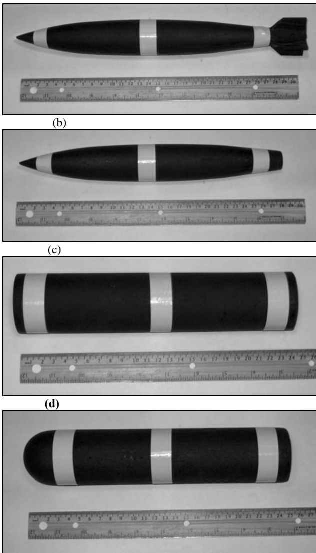
Figure 11. (a) MK-84 bomb models with 1/12 scale, (b) shell test model, (c) cylinder test model, and (d) capsule test model.
