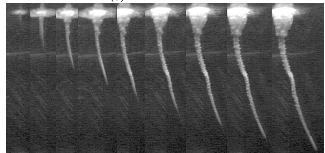
Figure 20. Model bomb trajectories from (a) Camera # 1, and (b) Camera #2.
