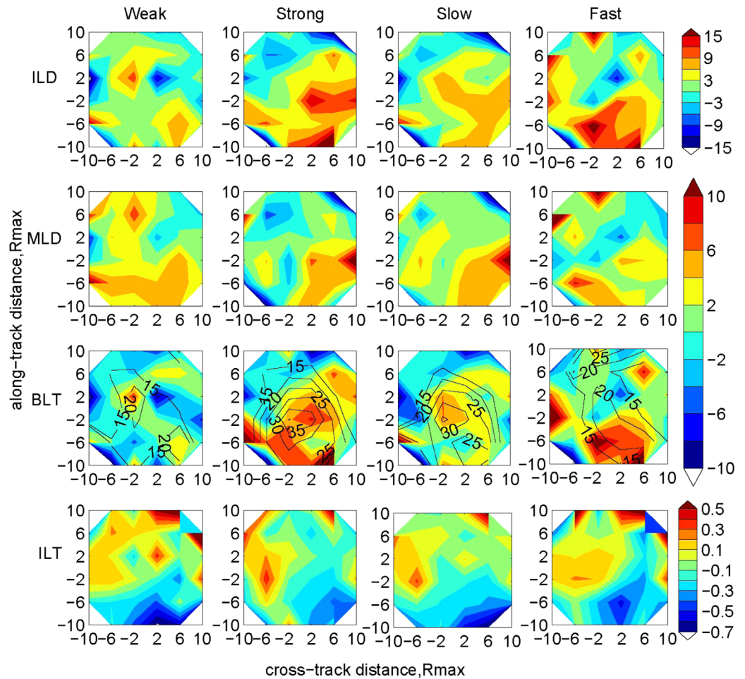
Figure 4. Instantaneous response of the ILD (m), MLD (m), BLT (m), and ILT (°C) during the weak, strong, slow, and fast TCs. Black contour indicates the averaged net freshwater flux (mm/d) from the 1 day before TC occurrence to the day of TC occurrence. Here R_{max} is the radius of TC's max winds with 47 km as the mean.
