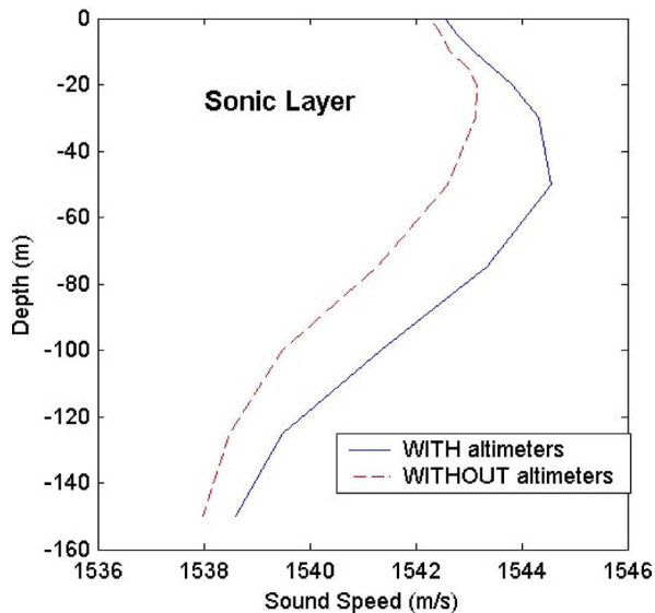
Fig. 16. Comparison of MODAS SSP at 32.5° N, 127.5° E on October 10, 2001 with and without satellite altimetry data assimilated. Note the existence of a sonic layer.
