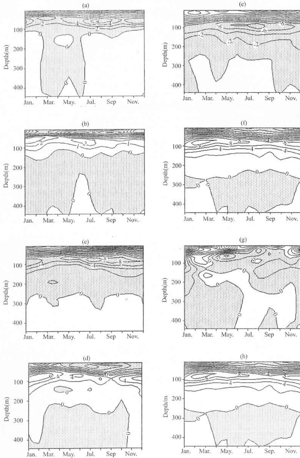
Fig. 5. Time-depth sections of meridional component of velocity(cm/s) along 1.352 3°N (left panels) and along 1.352 3°S (right panels)(Negative values are dotted). At 110°W(a,b), at 140°W(c,d), at 170°W(e,f) and at 165°E(g,h).
