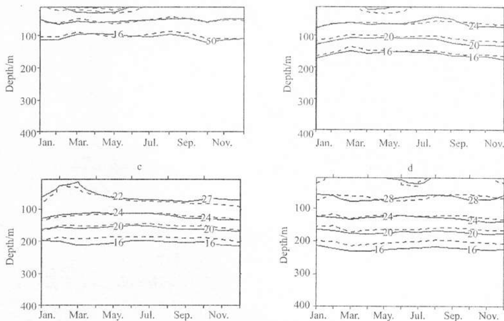
Fig. 3. Time-depth cross-sections of 14 a averaged temperature( ^{\circ}\text{C} ) along the equator observed from TOGA-TAO (dashed lines) and assimilated by SODA (solid lines) at 110^{\circ}\text{W} (a), at 140^{\circ}\text{W} (b), at 170^{\circ}\text{W} (c) and at 165^{\circ}\text{E} (d).
