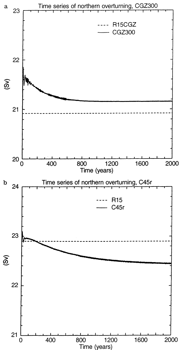
Fig. 7a,b. Time evolution of the northern overturning (in Sverdrup) at a location of ( 64^{\circ}\text{N} , 23507 m) for a CGZ300 and b C45r. See text for details about these runs
