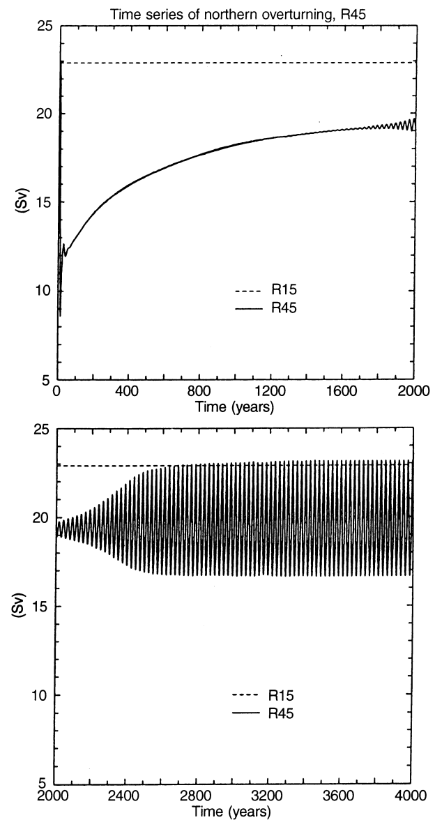
Fig. 8. Time evolution of the northern overturning (in Sverdrup) at a location of ( 64^{\circ}\text{N} , 2350 m) for R45
