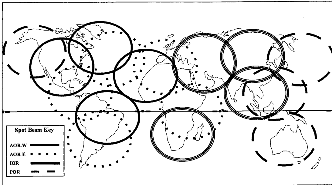
Figure 3-8. Inmarsat III Spot Beams. After Ref. [11].
